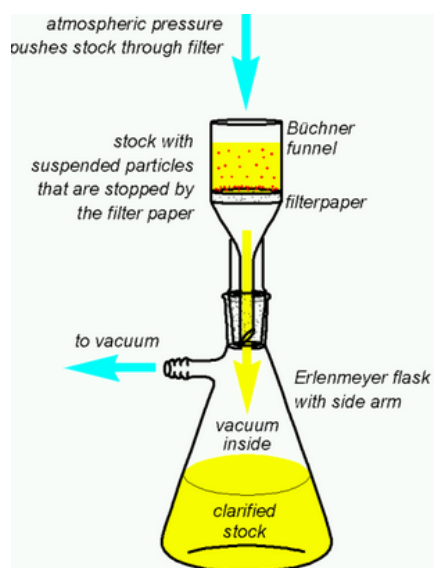
Vacuum filtration
