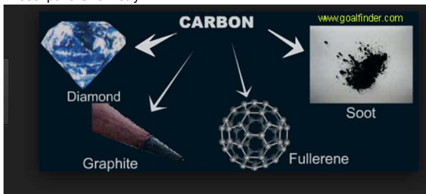
Carbon allotropes
